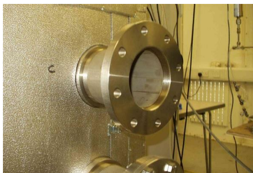
Figure 1: Stack simulator 5-inch port
